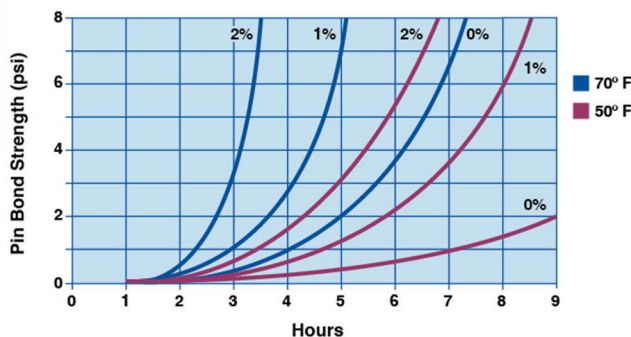
Figure 2. Concrete Hardening Rate with \text{CaCl}_2 Addition 1
