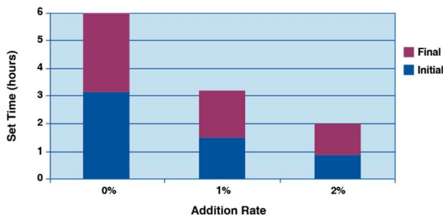
Figure 2. Concrete Hardening Rate with \text{CaCl}_2 Addition 1
